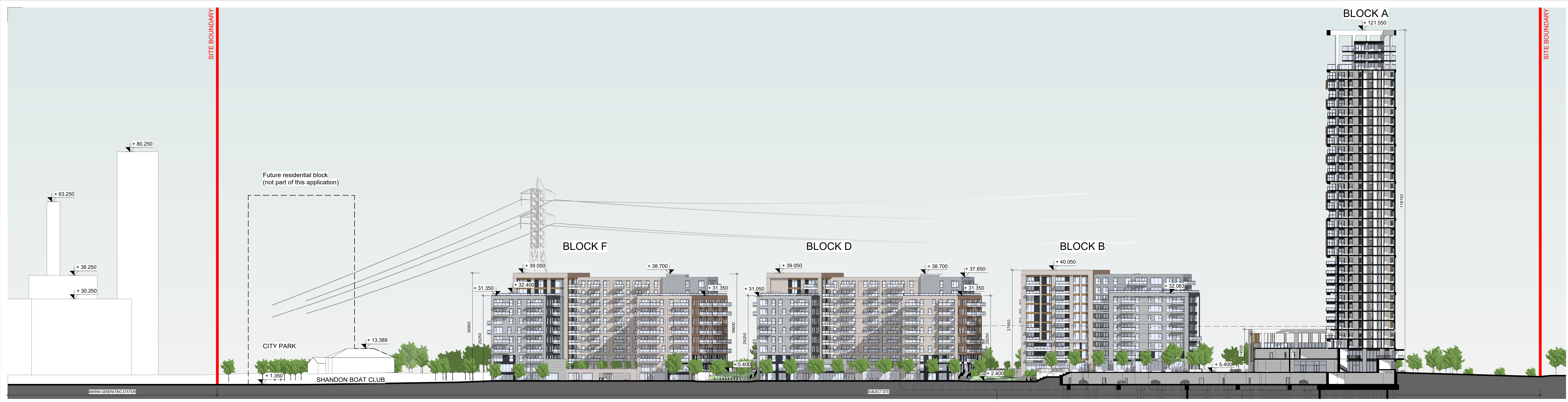
B PROPOSED CONTEXTUAL SITE SECTION B-B 1: 500
